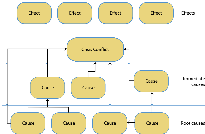
Figure 5: Problem Tree
